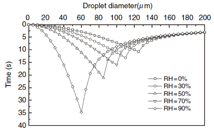
Fig. 6 Evaporation time and falling time of droplets of varying diameter under different atmospheric conditions ( T_{p0} = 33\text{ }^{\circ}\text{C} , T_{\infty} = 18\text{ }^{\circ}\text{C} )
