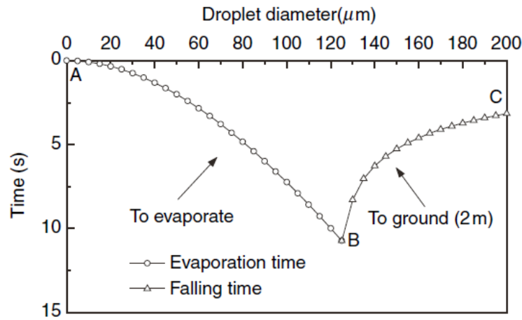
Fig. 5 Evaporation time and falling time of droplets of varying diameter ( T_{p0} = 33\text{ }^{\circ}\text{C} , T_{\infty} = 18\text{ }^{\circ}\text{C} , \text{RH} = 0\% )
